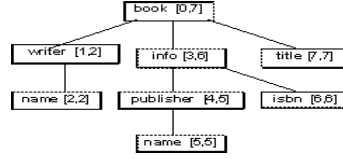
Fig. 1. XML schema tree with labels and [node number, node scope] for each node
