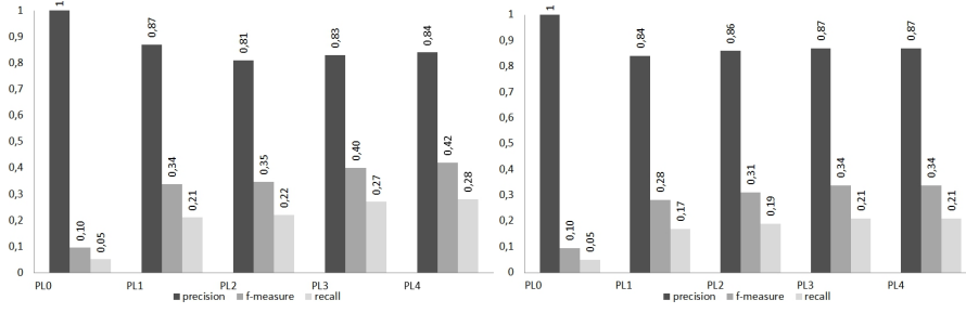
Fig. 6 precision and recall for “All Ontologies” (1-context and 2-context traversal) and “Selected Ontologies” (1-context and 2-context traversal) and conjunctive aggregation of alignments.
